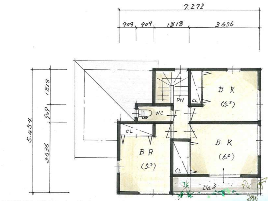
2F PLAN
